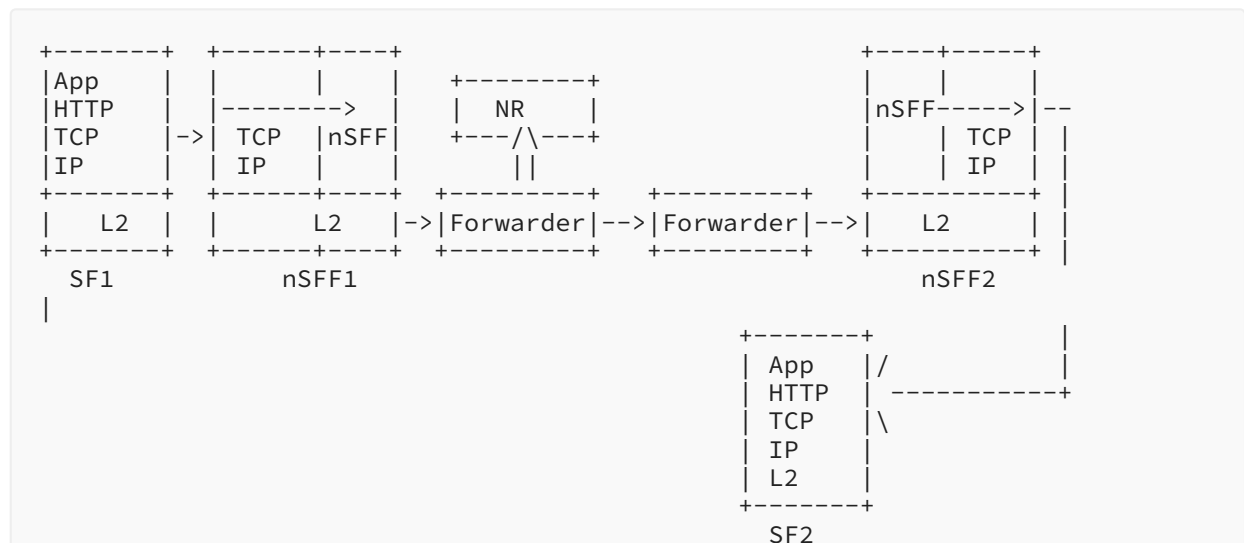
Figure 4: Protocol Layers
